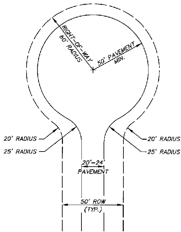
CUL-DE-SAC DETAIL NOT TO SCALE
